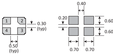
SOLDER PAD LAYOUT
