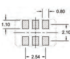
Figure 2) Top, Side, Bottom & Land
