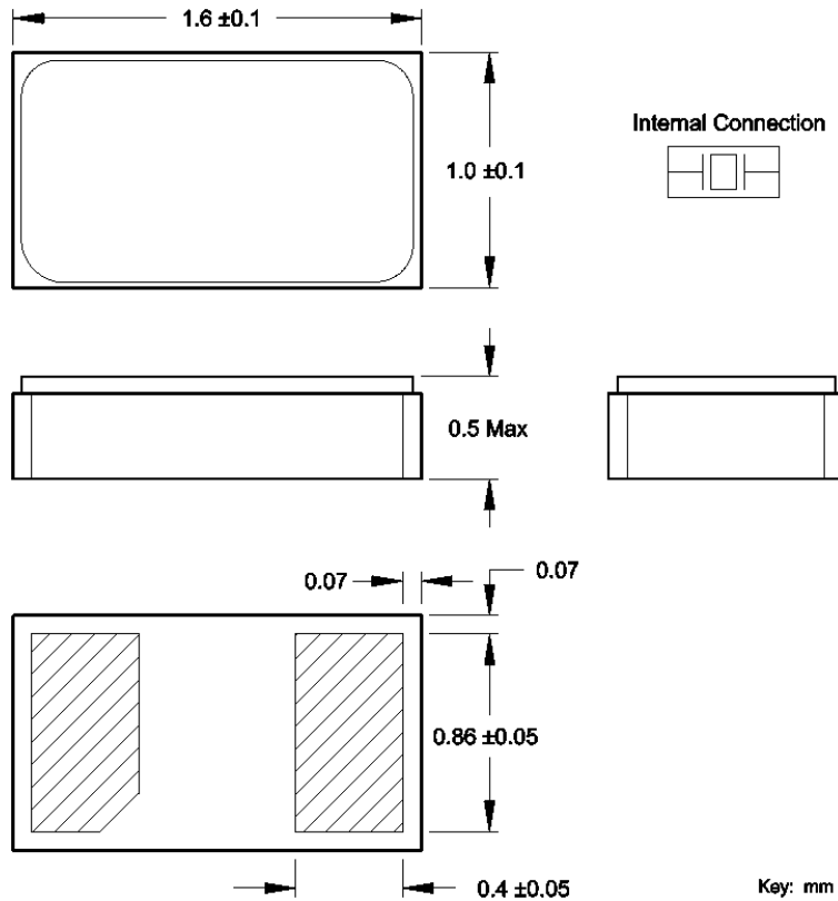
Package Drawing
