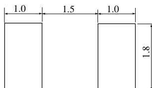
Recommended Solder Pattern
