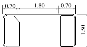
Recommended Solder Pattern
