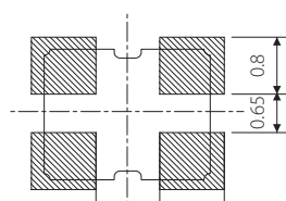
Example of a Terminal Land Pattern
